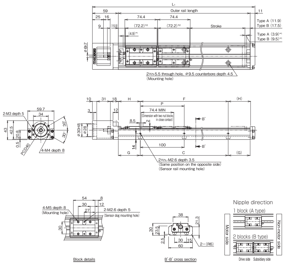
Block details
