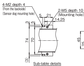
Sub-table details
