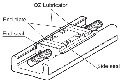
Appearance Drawing
